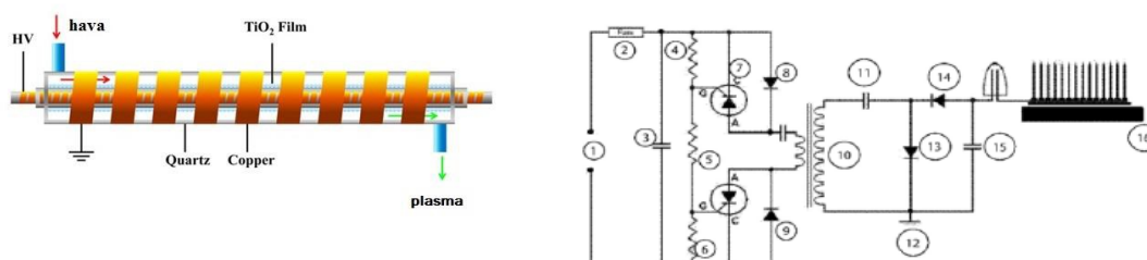
Fig. 1. Schematic of the nano-plasma air purification device.
